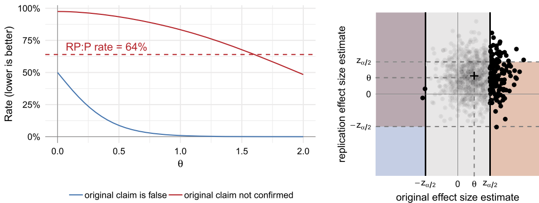
(a) The expected fraction of replications that do not confirm (at level 0.05) the original directional claim (red) and the proportion of false directional claims in the original studies (blue), as a function of effect size \theta . For small \theta , the fraction of replications that do not confirm the claims in the original studies may dramatically overestimate the fraction of false original claims. (b) \theta = 1 . The gray region is unobserved. For points in the red region, the replication does not confirm the original directional claim; for points in the blue region, the original claim is directionally false. The red and blue regions overlap in the purple region.
