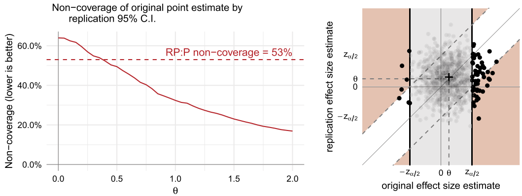
(a) Expected fraction of original point estimates falling outside the replication confidence interval, as a function of effect size \theta . For small \theta , the fraction of original point estimates falling outside the replication 95% confidence intervals can easily exceed the RP:P reported metric of 53%, even when all replications are perfectly exact. (b) \theta = 0.5 . The gray region is unobserved. For points in the red region, the original point estimate differs from the replication estimate by more than z_{\alpha/2} , and, hence, the original point estimate falls outside in the replication 95% confidence interval.
