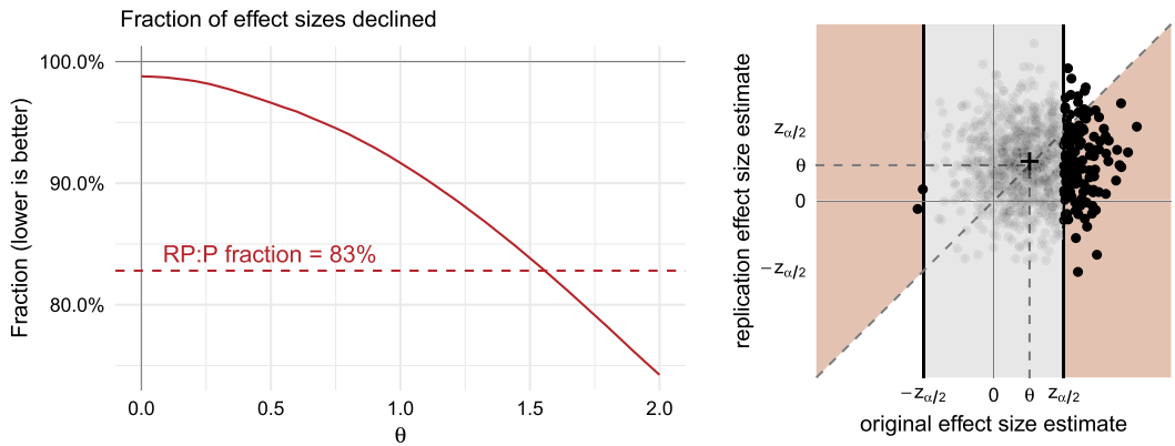
(a) Expected fraction of effect size point estimates that declined toward zero in replication as a function of effect size of \theta . For small \theta , the fraction of effect size estimates declining from original to replication studies can easily exceed the RP:P reported metric of 83%, even when there is no decline in the true effect sizes. (b) \theta = 0.5 . The gray region is unobserved. Points in the red region represent declining point estimates in replications. When the original point estimate is positive, a decline is marked by a smaller replication estimate; on the other hand, if the original estimate is negative, a decline is indicated by a larger replication estimate.
